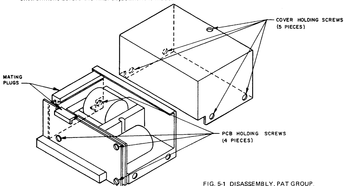
FIG. 5-1 DISASSEMBLY, PAT GROUP.
